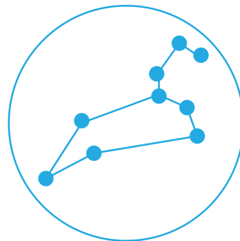
Leo
