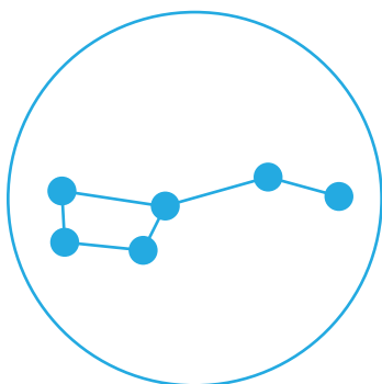
Osa Mayor
