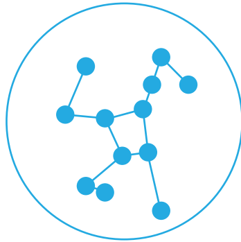
Hércules
