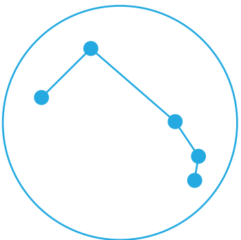
Aries
