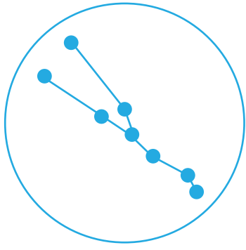
Tauro
